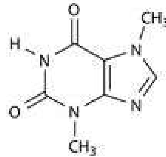
Theobromine
